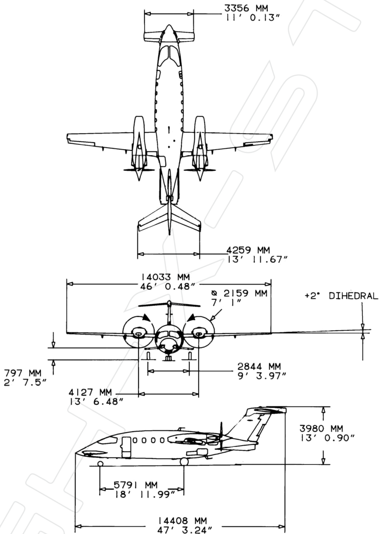
Figure 1: 3-view drawing of the Piaggio P.180 Avanti
